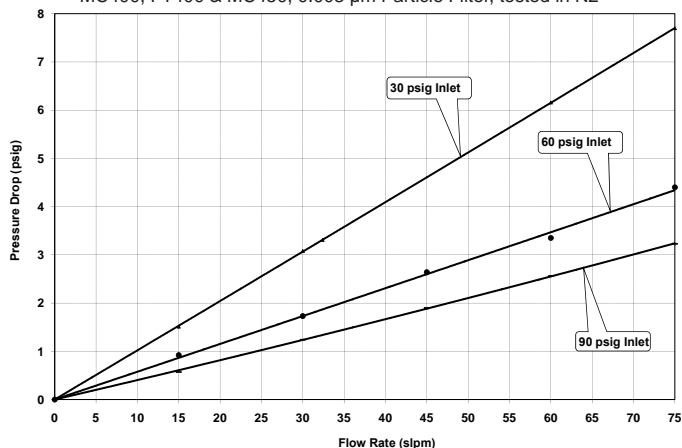
Pressure Drop vs. Flow Rate MC400, FT400 & MC450, 0.003 µm Particle Filter, tested in N2
